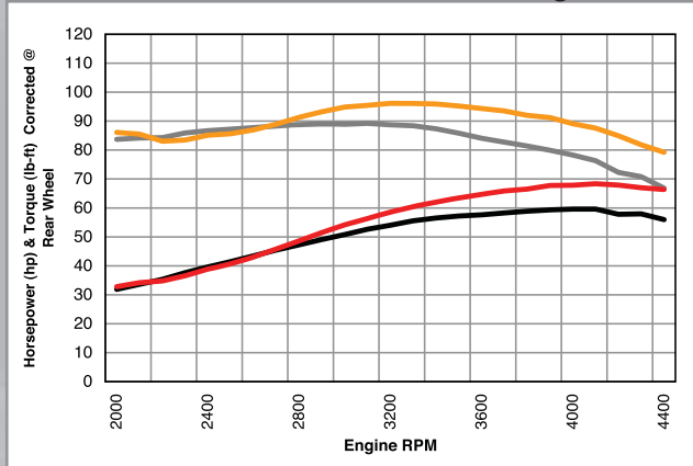
'08~'10 Road Star - Stock vs. Stage II
