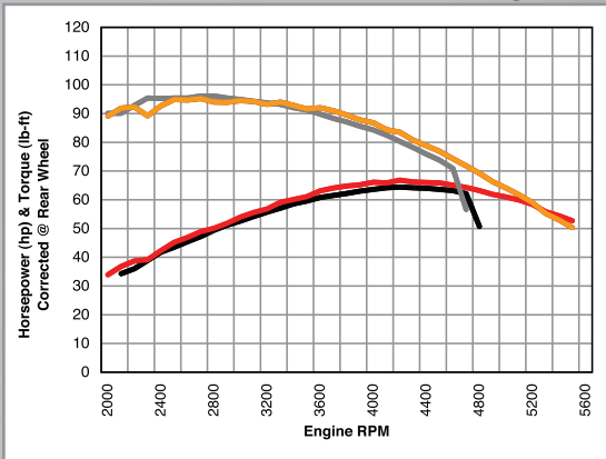
'04~'07 Road Star - Stock vs. Stage II
