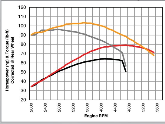
'04~'07 Road Star - Stock vs. Stage IV
