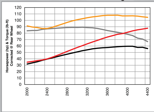
'08~'10 Road Star - Stock vs. Stage III
