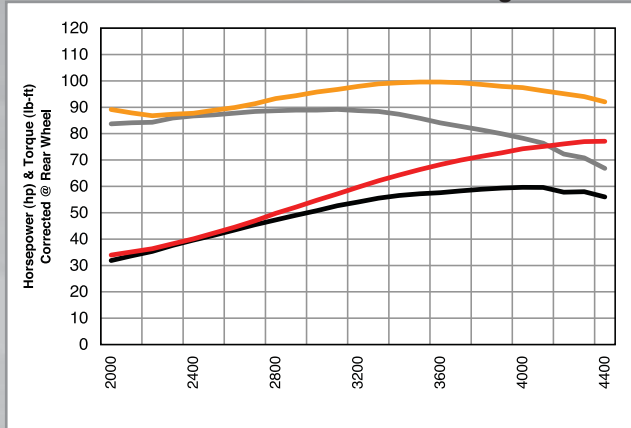
'08~'10 Road Star - Stock vs. Stage III
